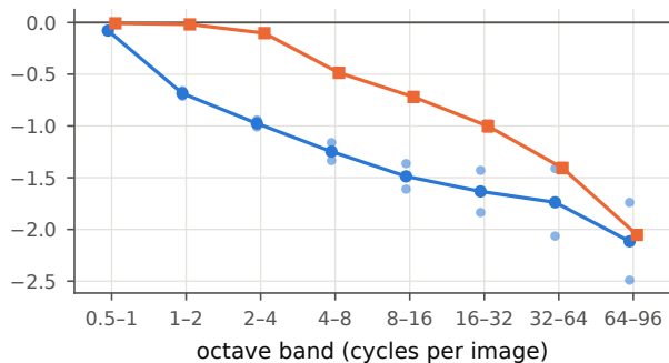
LSUN Bedrooms
