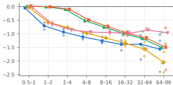
LSUN Bedrooms
