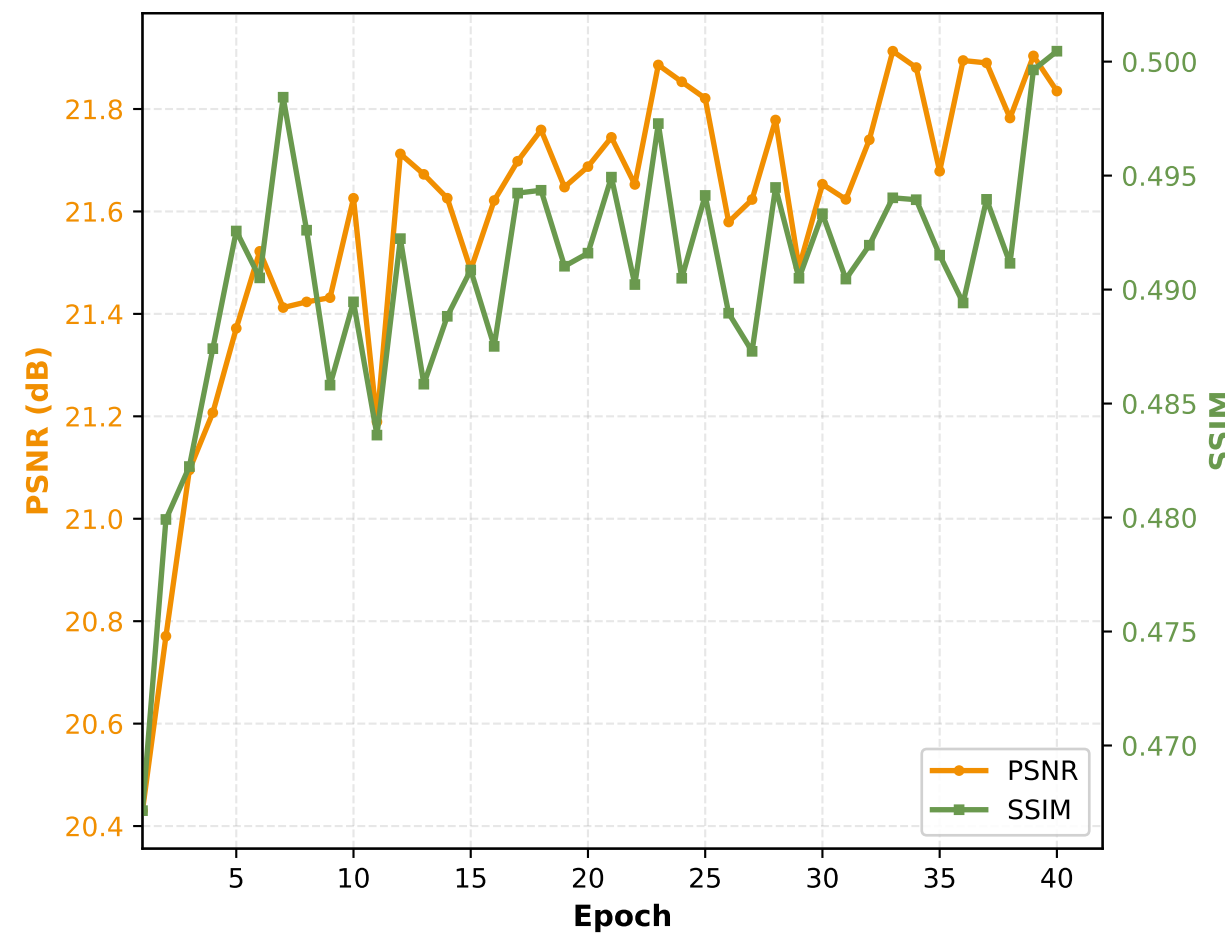
Quality Metrics (Validation)
