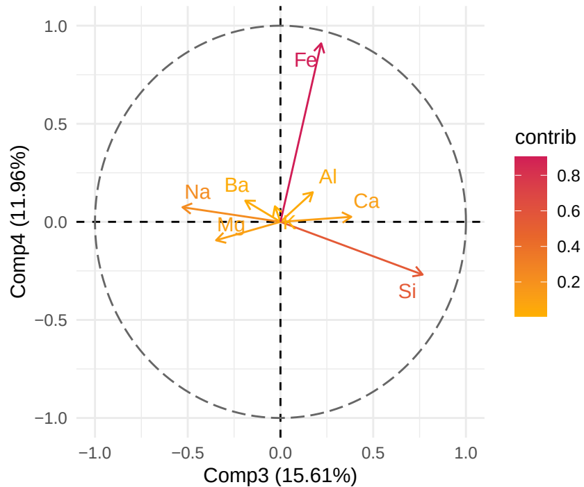
Correlation Plot
