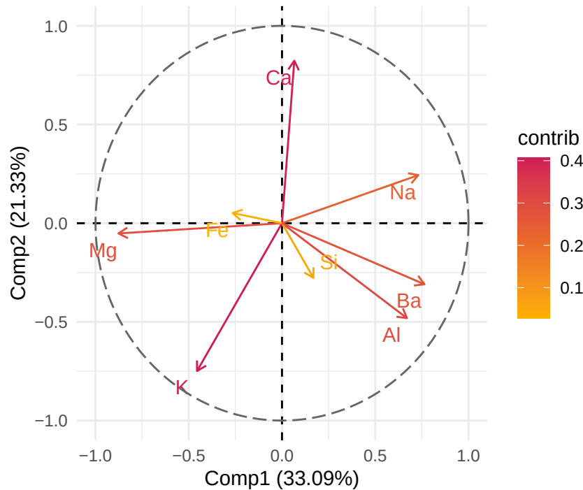
Correlation Plot
