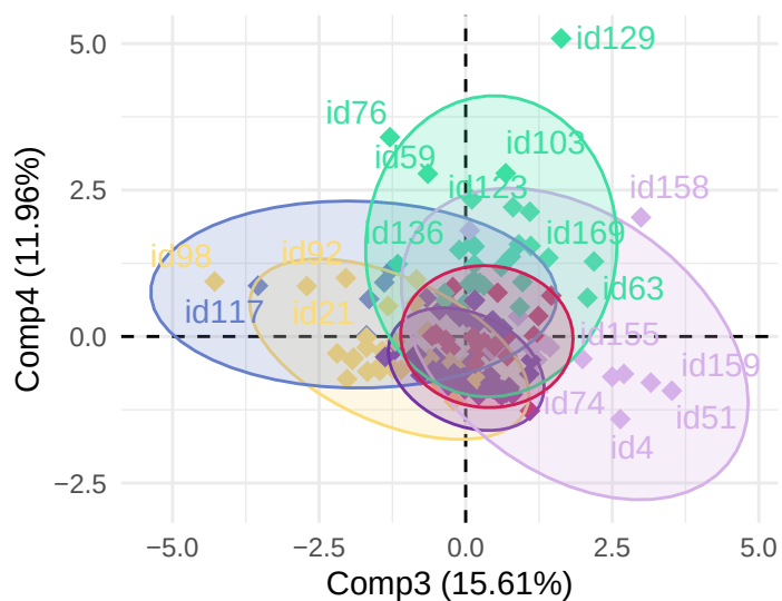
Score Plot
