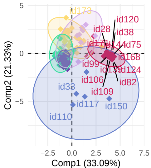
Score Plot
