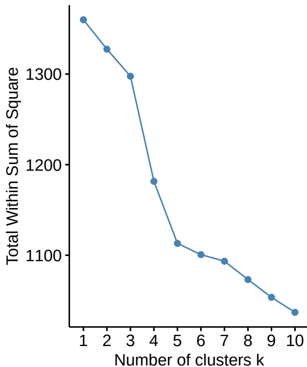
WSS (codo)
