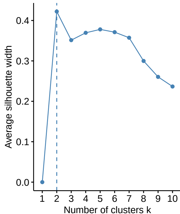
Silhouette
