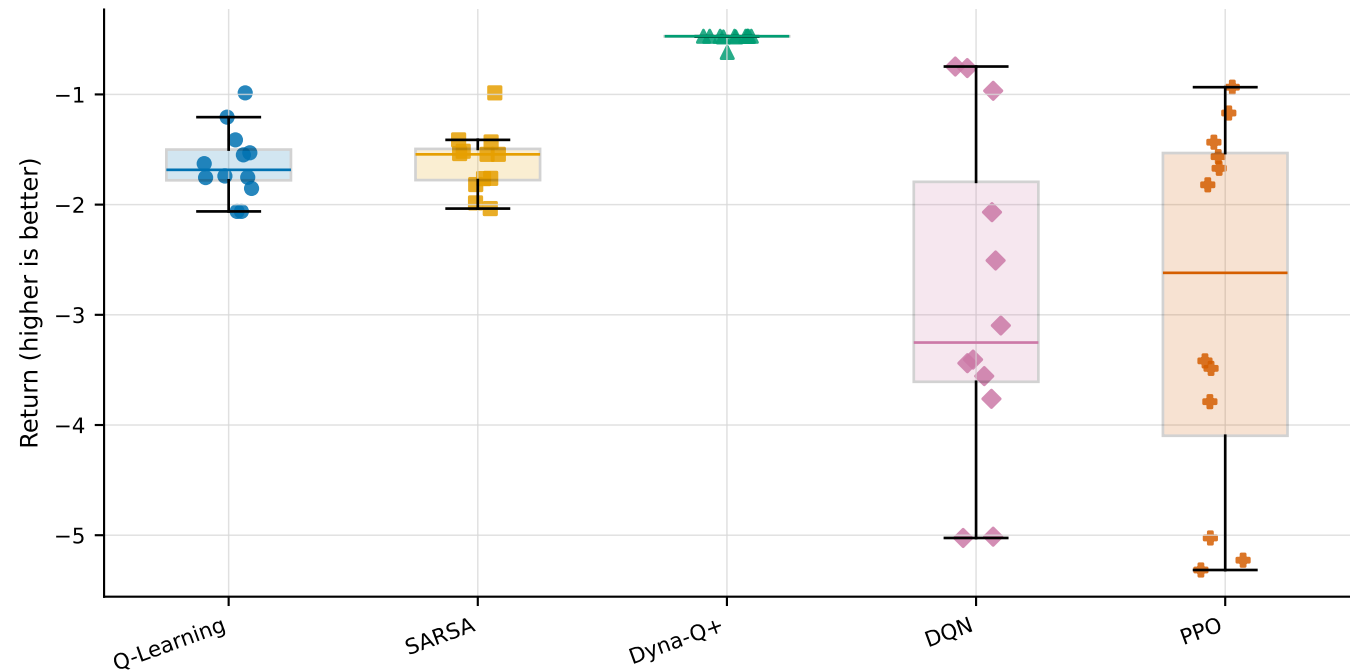
RQ1 root-level time-average distribution
