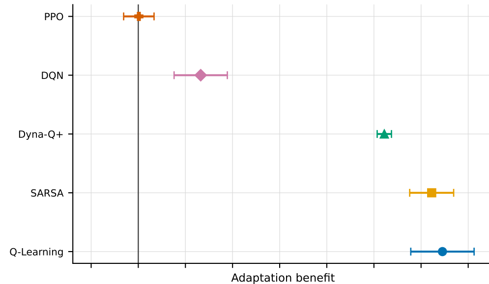
Action failure 0.15
