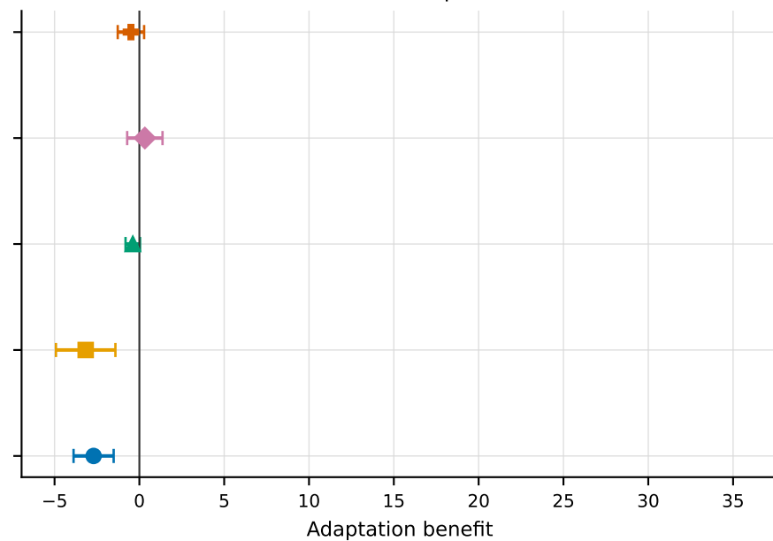
Observation corruption 0.05
