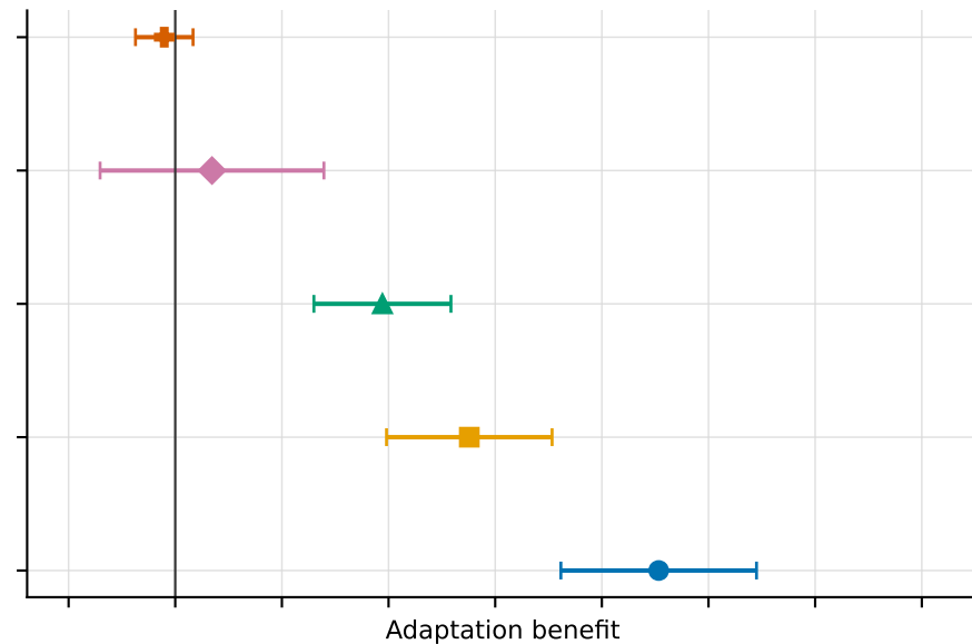
Observation corruption 0.05
