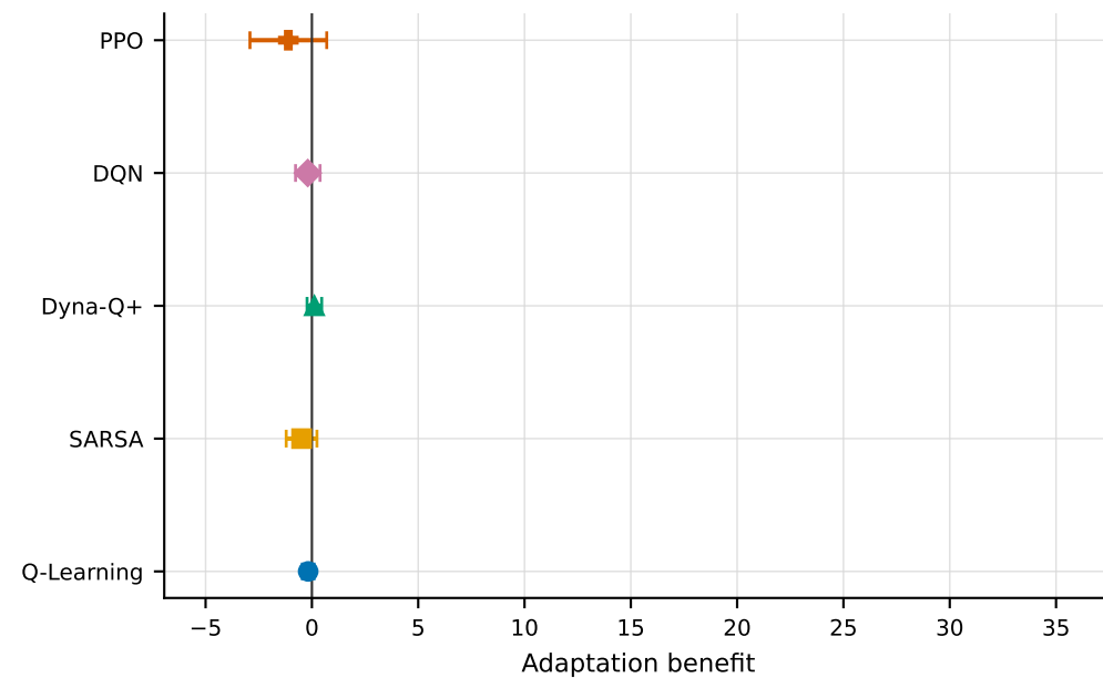
Action failure 0.15
