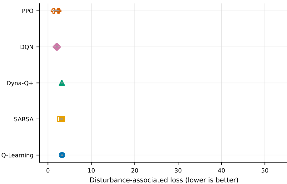
Action failure 0.15
