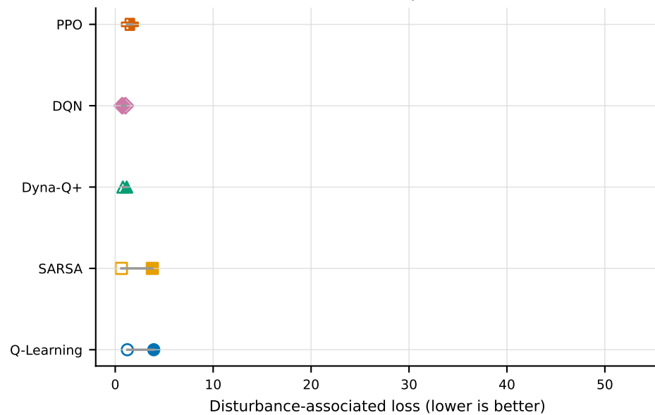
Observation corruption 0.05
