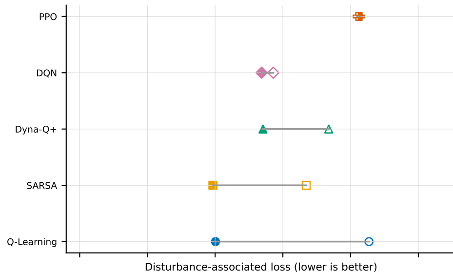
Observation corruption 0.05
