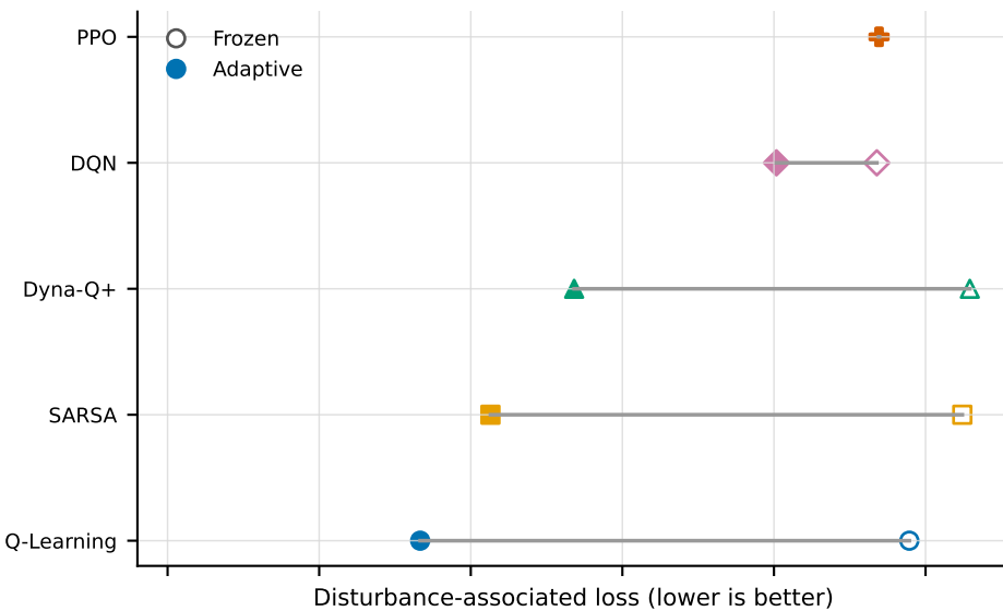
Action failure 0.15
