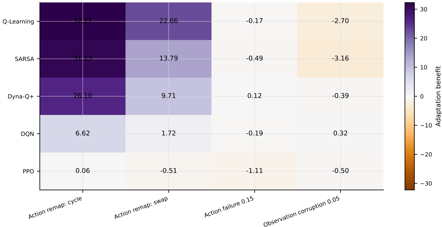
RQ2 adaptation benefit (higher is better)
