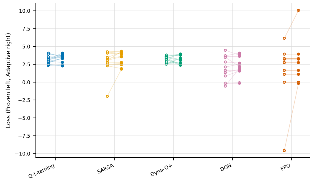
Action failure 0.15
