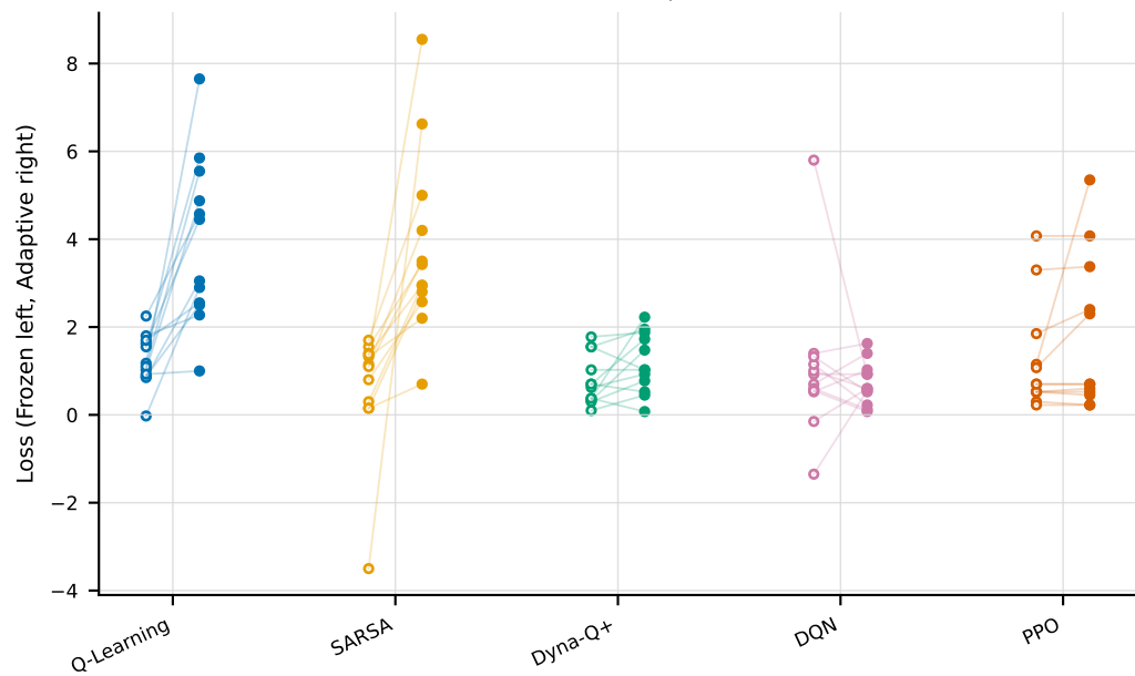
Observation corruption 0.05
