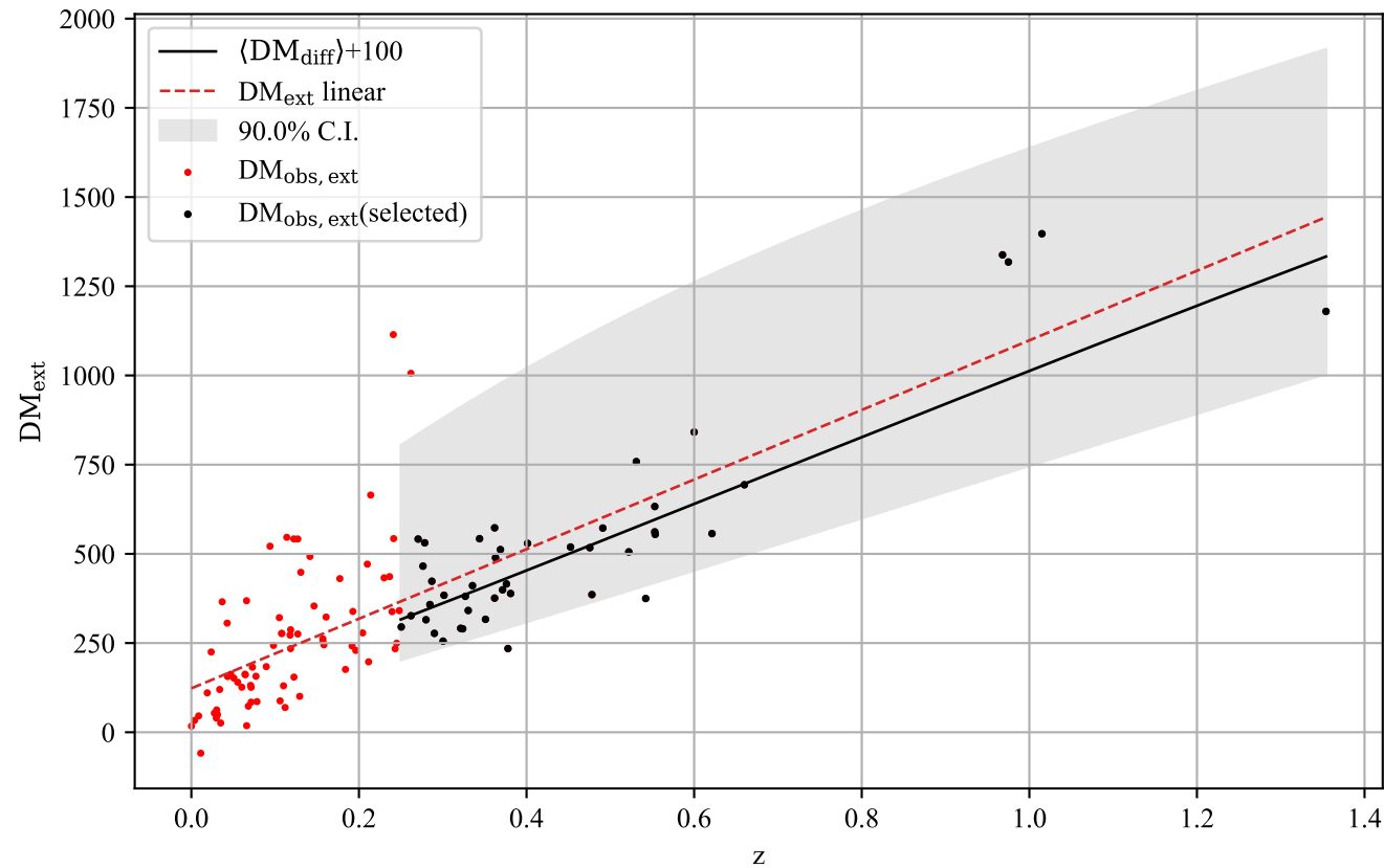
FRB z-DM relation
