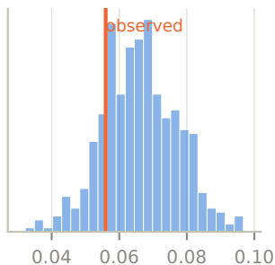
(b) HCP: clustering p = 0.836
