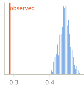
(c) HCP: strength CV p = 1.000
