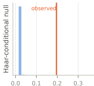
(a) HCP: IPR p = 0.004
