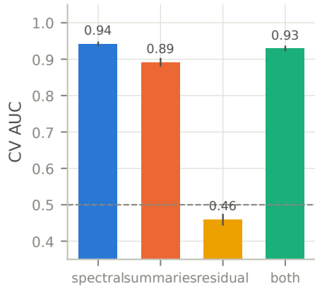
(a) rotatable cohort: signal in spikes
