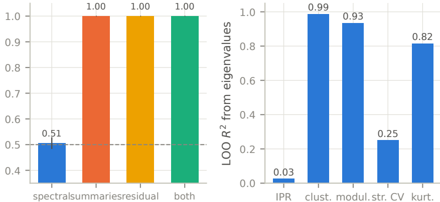
(b) non-rotatable cohort: signal in eigenvectors S&P 500: summaries from eigenvalues
