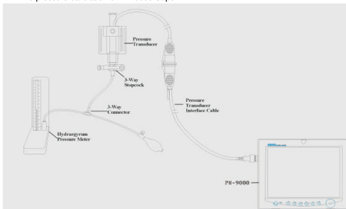
Figure 5-5 IBP Calibration
