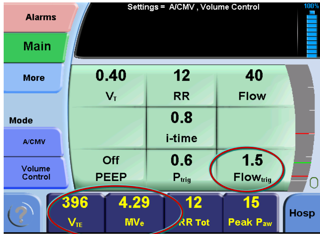
With Flow Sensor
