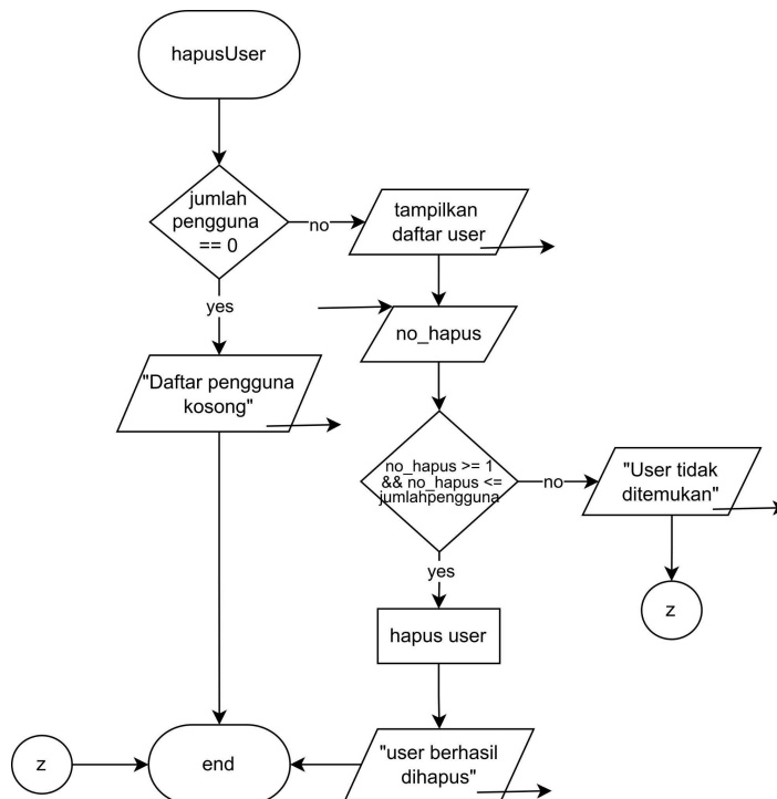
Gambar 2.12.1 flowchart hapusUser
