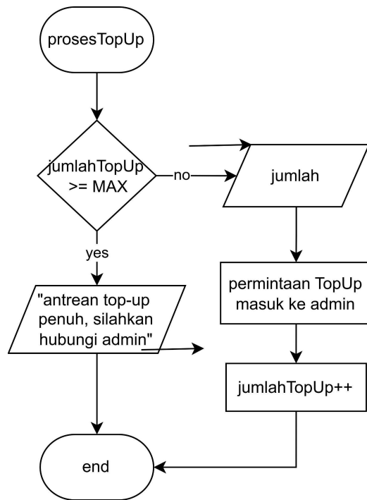
Gambar 2.16.1 flowchart prosesTopUp
