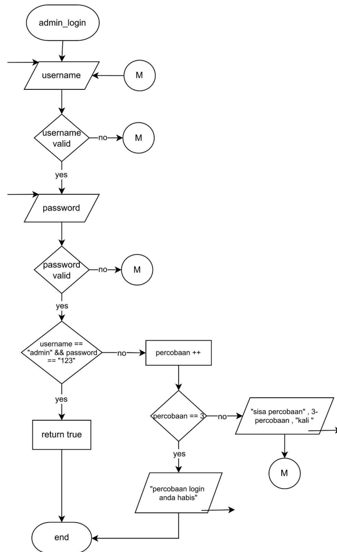
Gambar 2.2.1 flowchart admin_login
