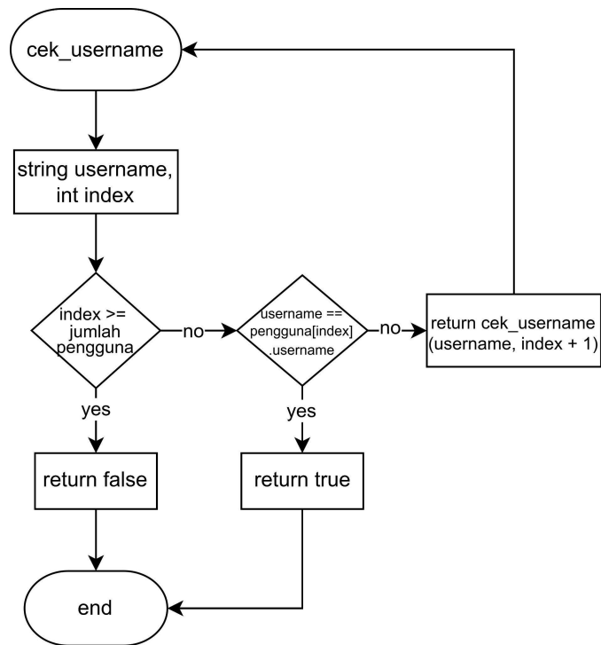
Gambar 2.4.1 flowchart cek_username
