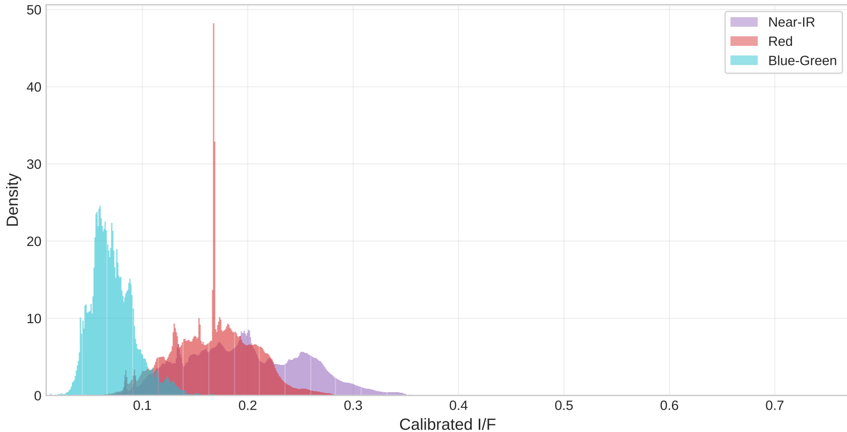
Mars HiRISE Channel Intensity Distributions
