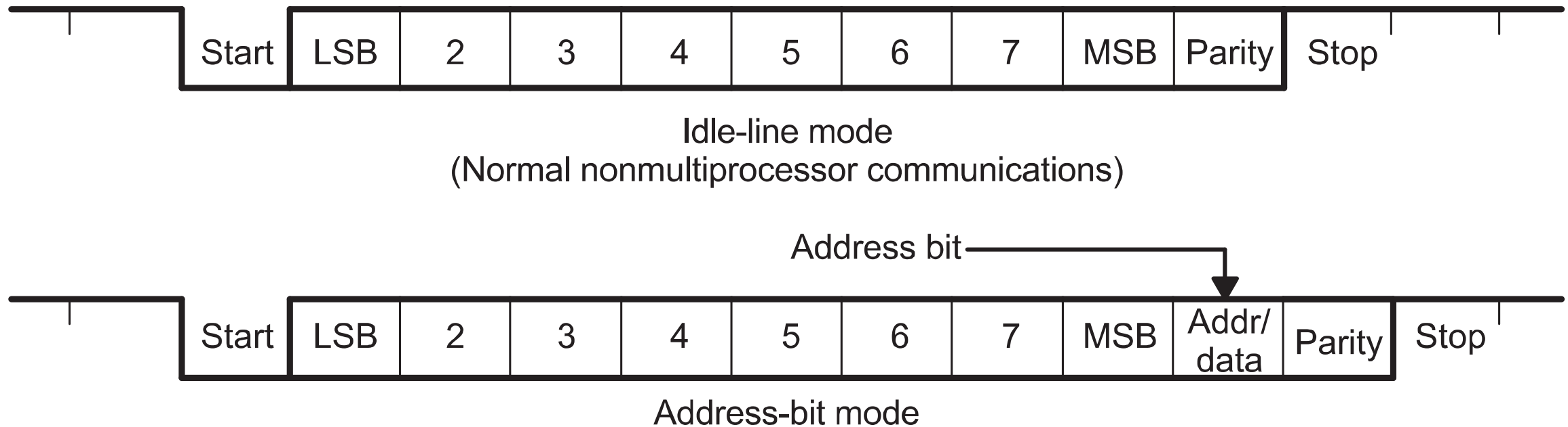
Figure 19-3. Typical SCI Data Frame Formats
