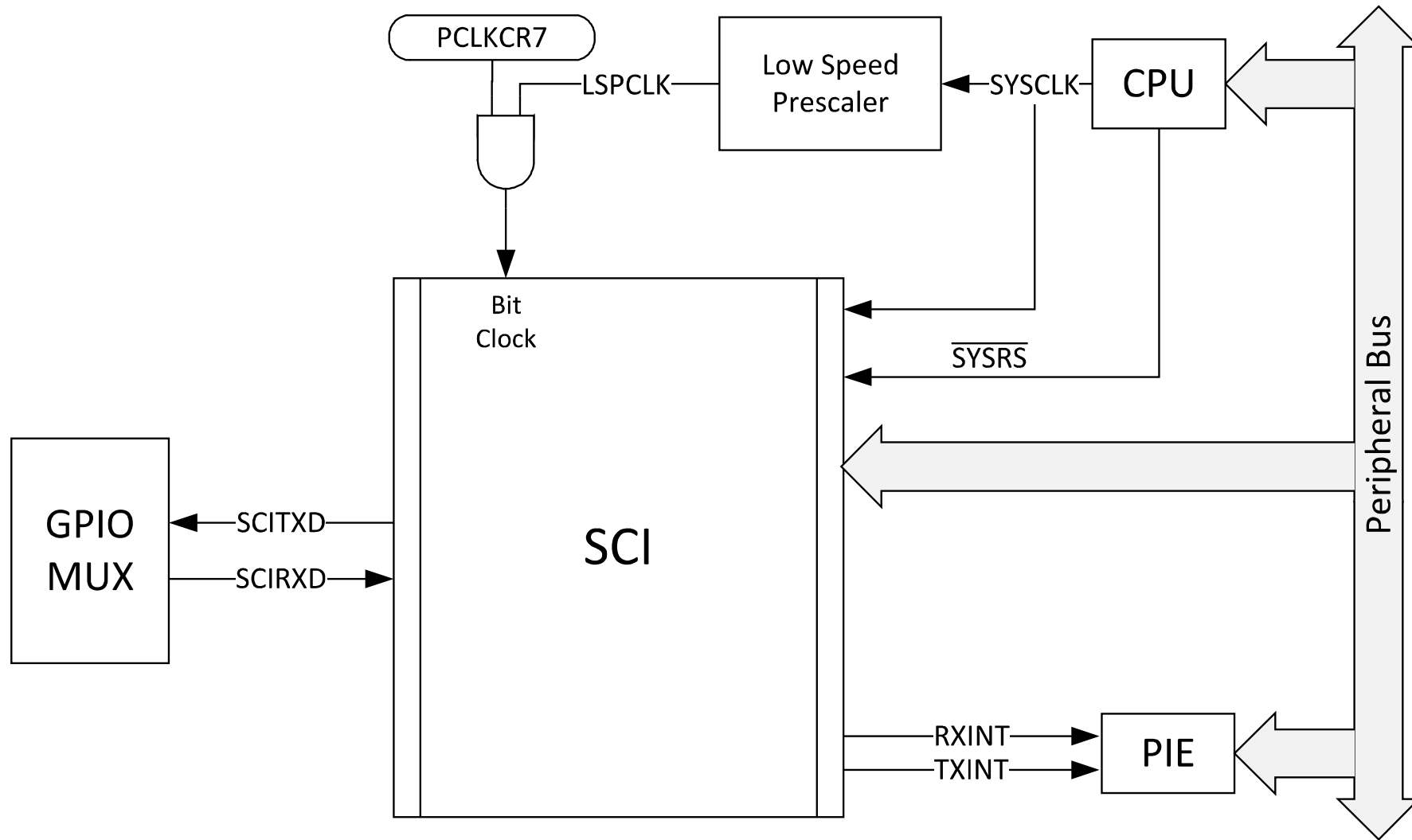
Figure 19-1. SCI CPU Interface
