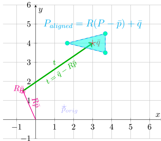
Step 4: Translation t ( t = \bar{q} - R\bar{p} )
