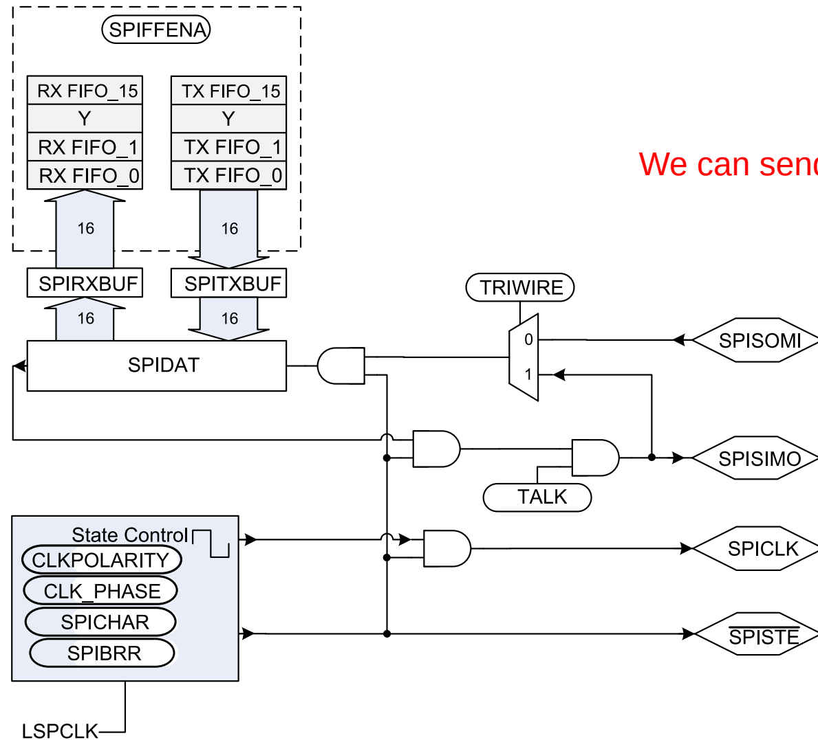
Figure 18-5. SPI Module Master Configuration
