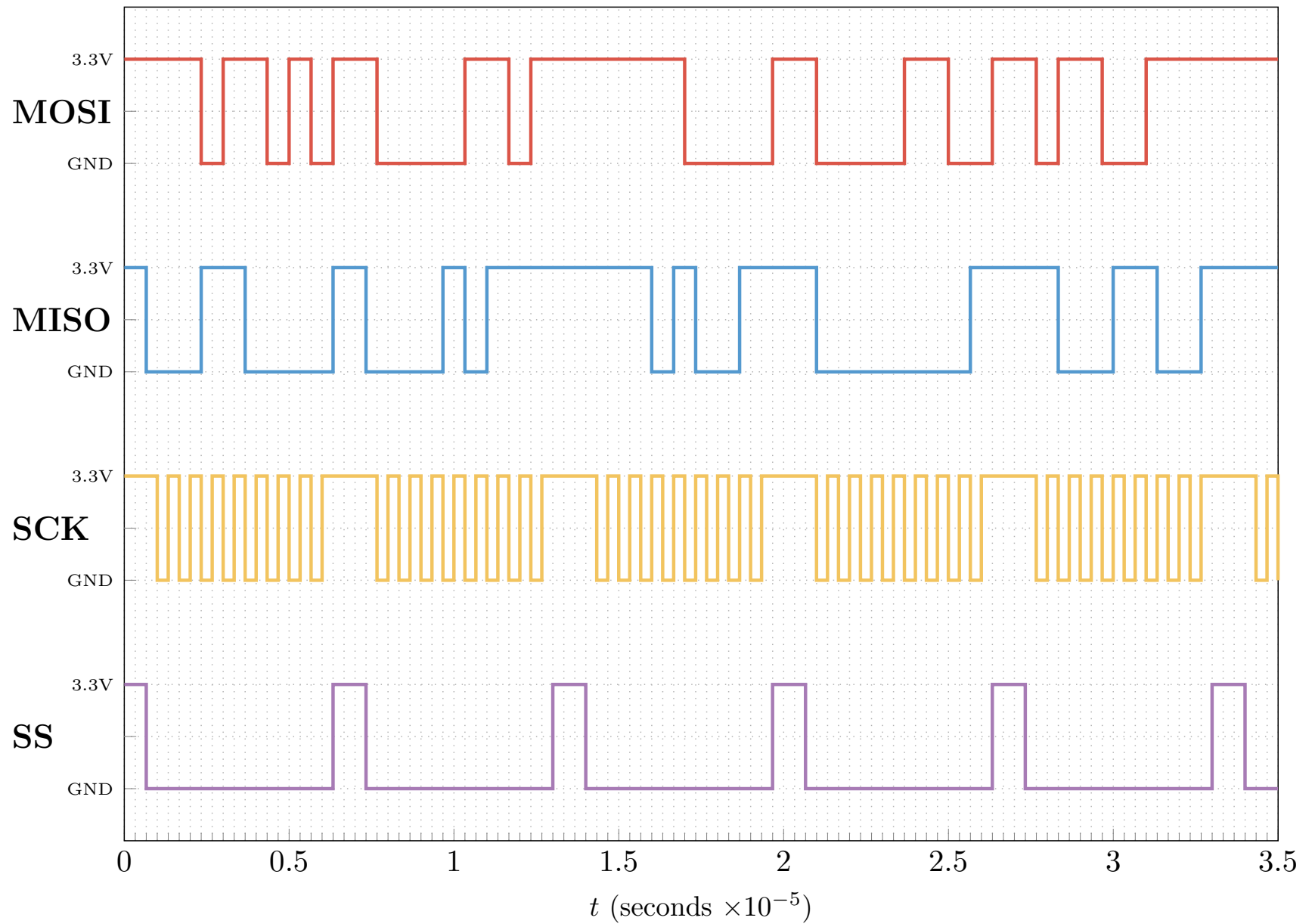
Figure 3: SPI Timing Diagram Analysis
