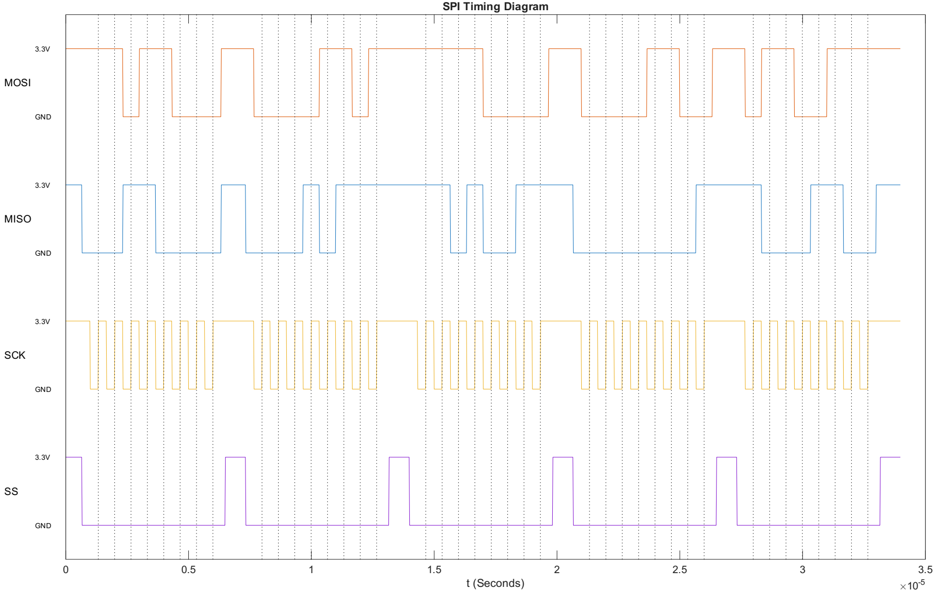
Figure 3: SPI Timing Diagram Analysis
