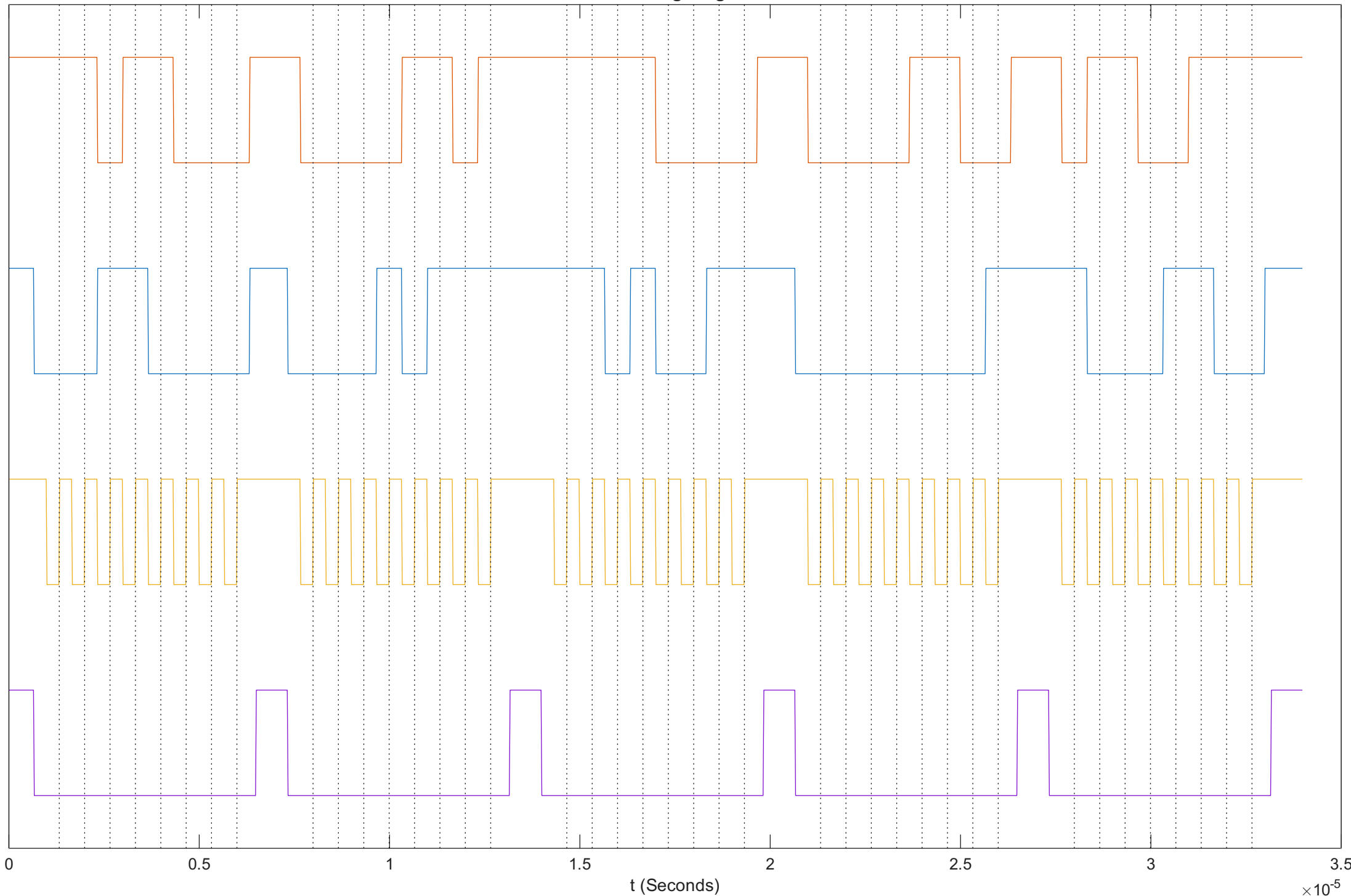
SPI Timing Diagram
