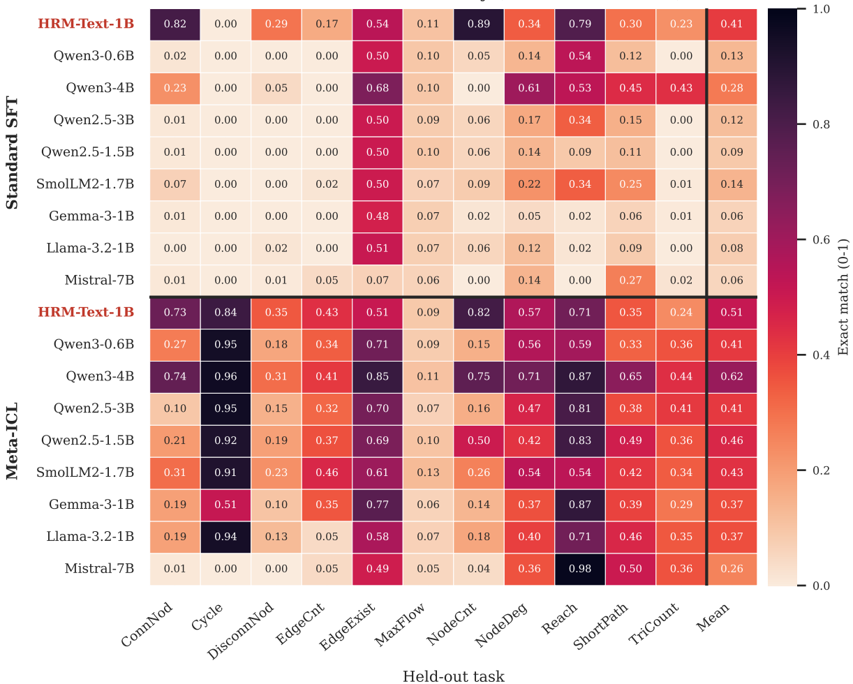
Out-of-distribution accuracy (leave-one-task-out)
