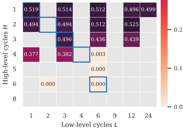
Full backprop
