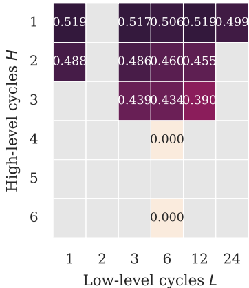
Truncated BPTT (5 blocks)
