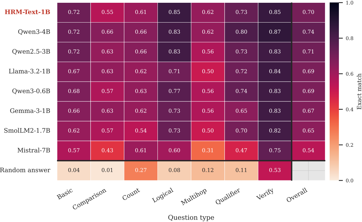
KQA-Pro exact match by question type
