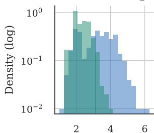
Mean shortest path
