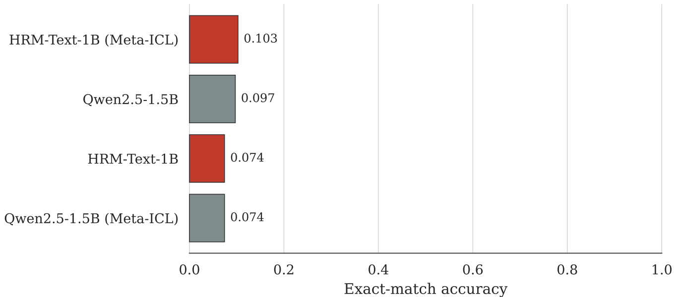
Out-of-distribution performance (MaximumFlow)
