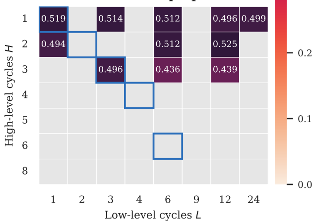
Full backprop
