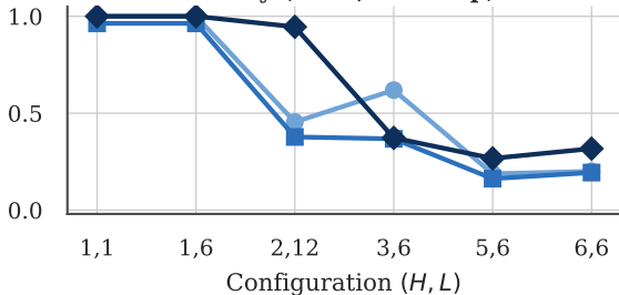
Token accuracy (train, last step)
