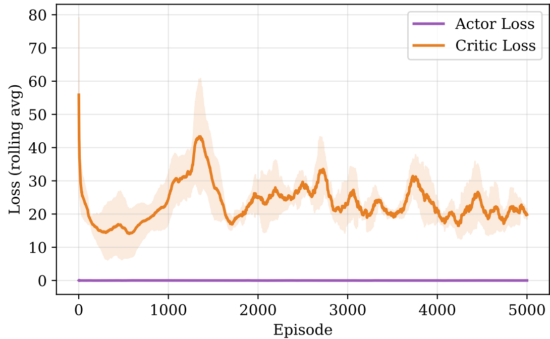
Actor-Critic Losses
