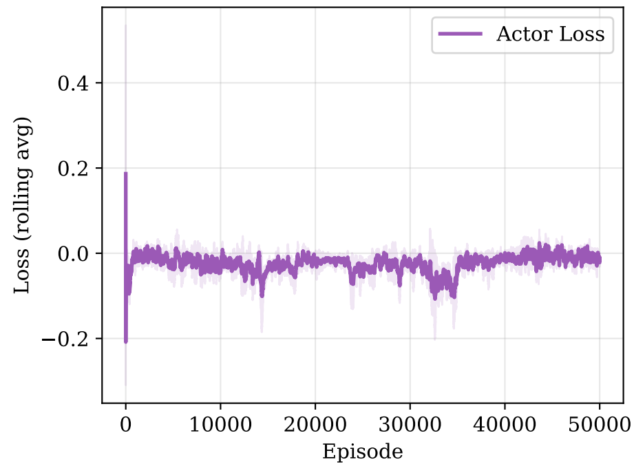
Actor-Critic Actor Loss
