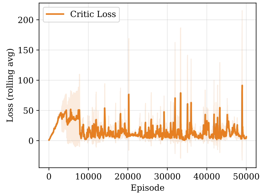
Actor-Critic Critic Loss
