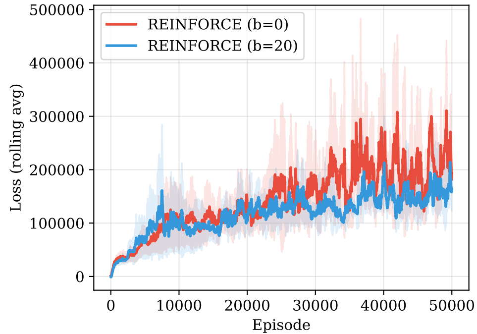
REINFORCE Loss
