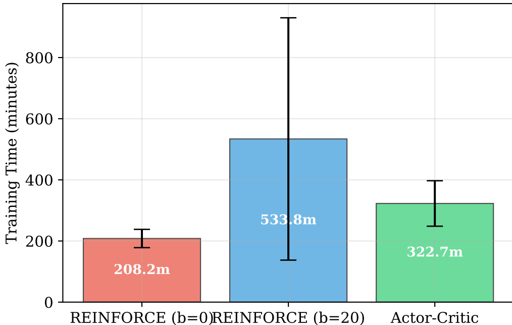
Training Time Comparison
