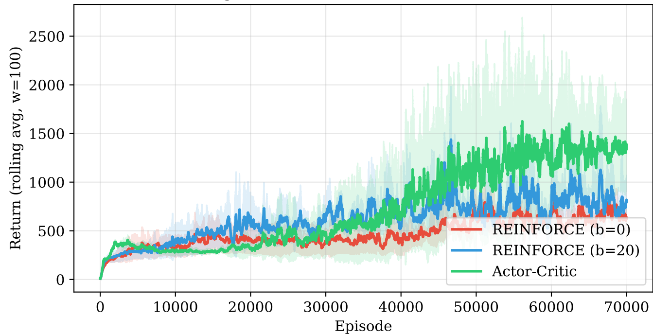
Learning Curves — REINFORCE vs Actor-Critic
