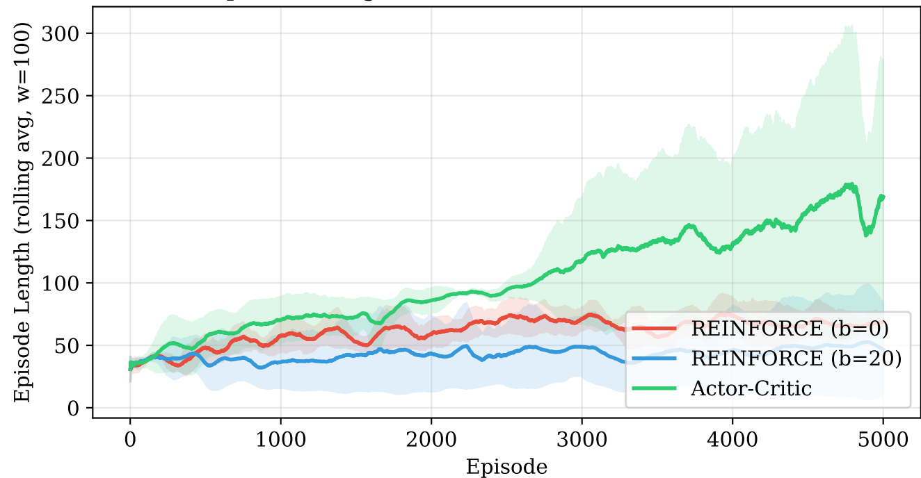
Episode Lengths — REINFORCE vs Actor-Critic
