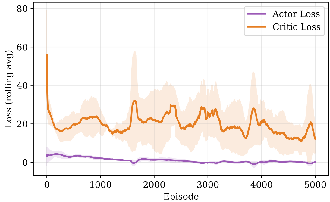
Actor-Critic Losses
