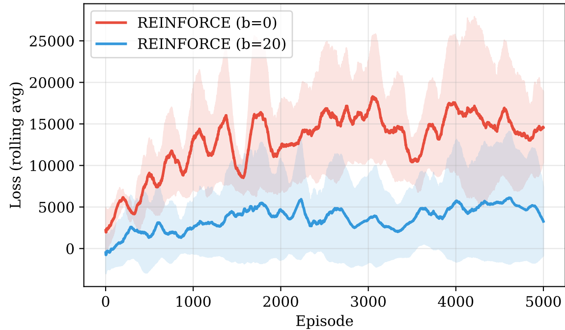
REINFORCE Loss
