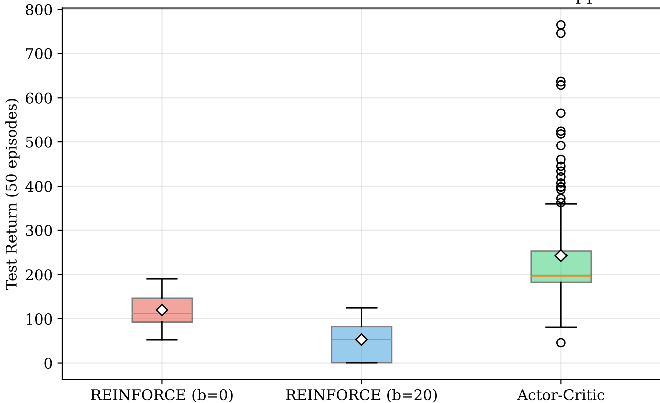
Test Performance — REINFORCE vs Actor-Critic on Hopper-v4
