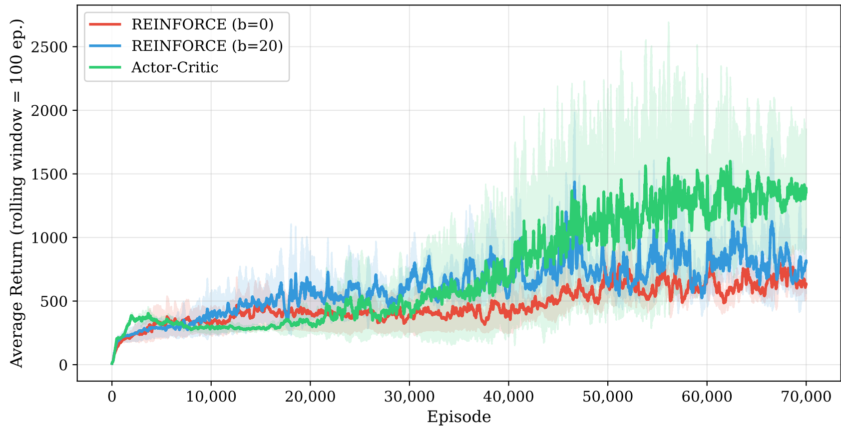
Training Performance: Average Reward \pm Std over Seeds
