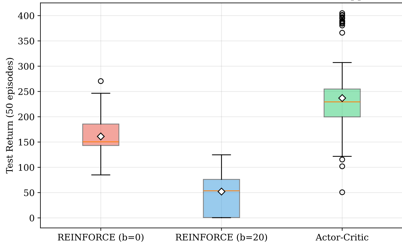
Test Performance — REINFORCE vs Actor-Critic on Hopper-v4
