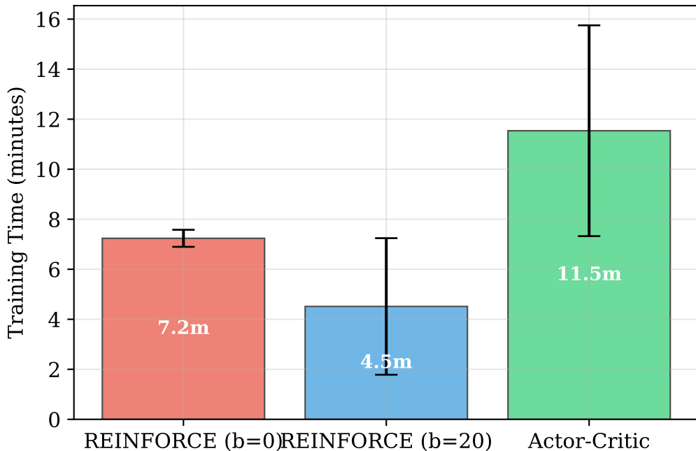
Training Time Comparison
