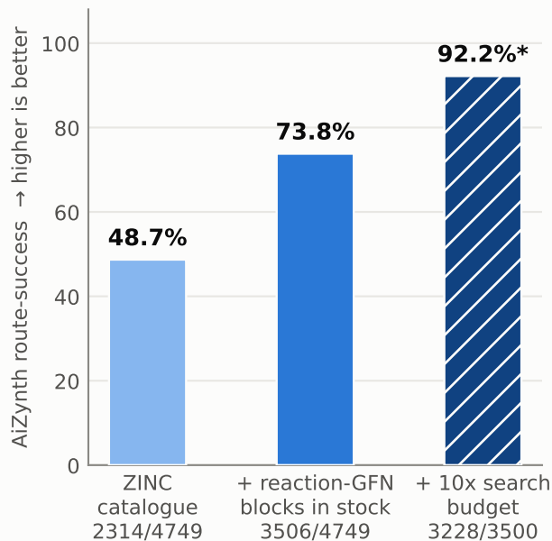
C Are the molecules makeable?
