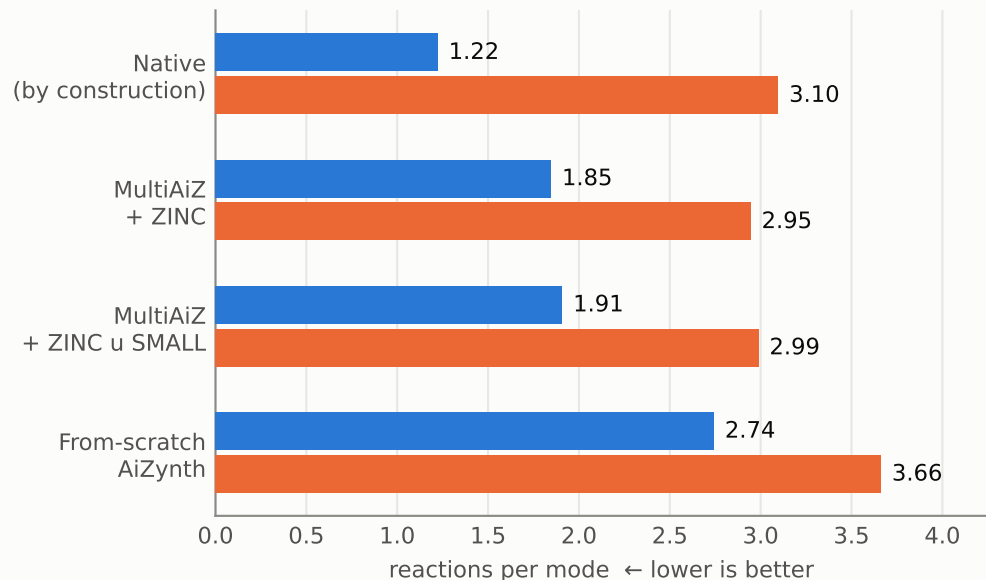
A Route cost by pricing regime
