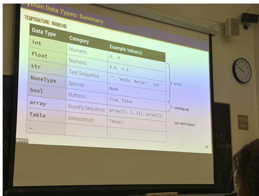
Figure 3: Data Types
