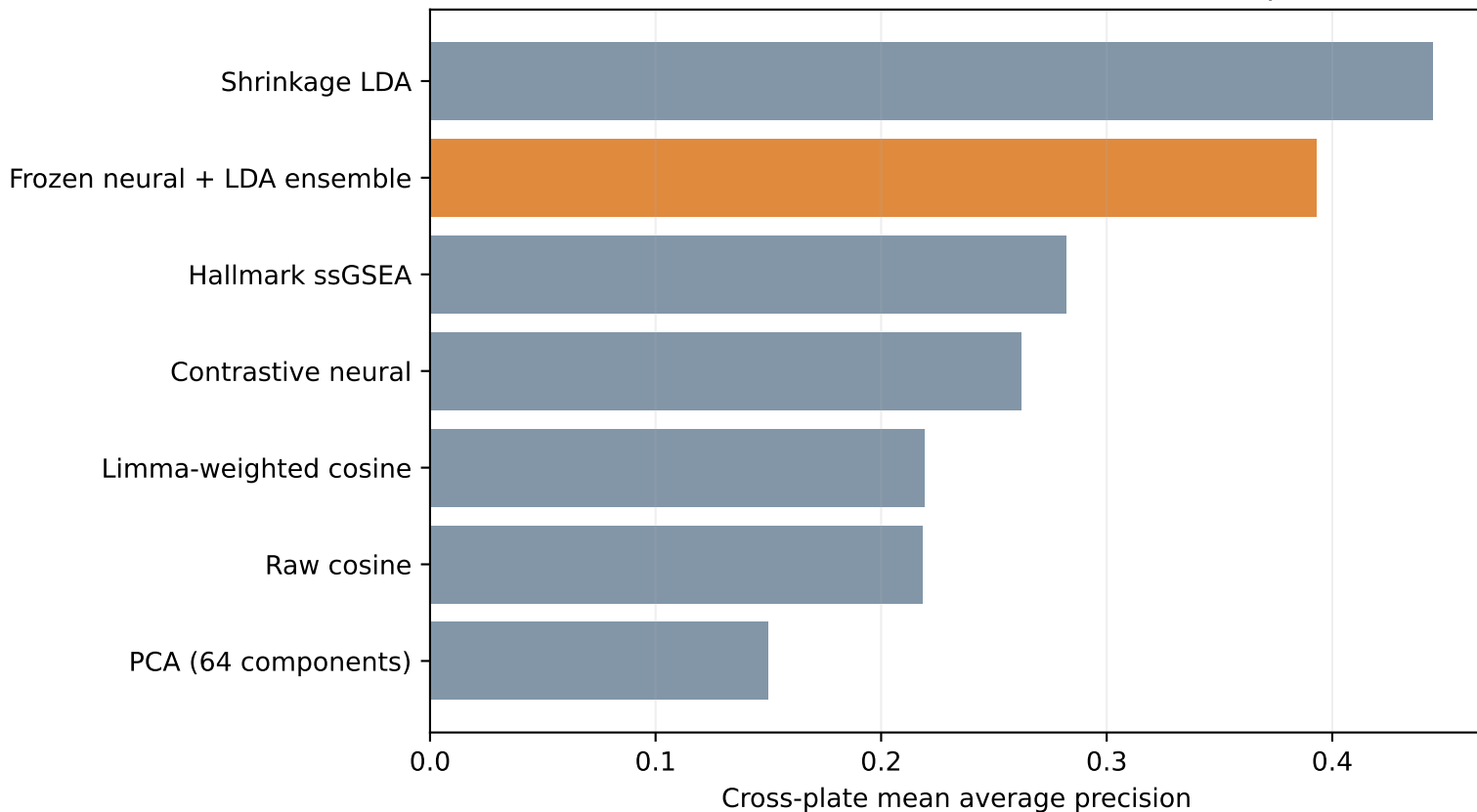
Frozen external validation: GSE70138 MCF7, 10 \mu M, 24 h
