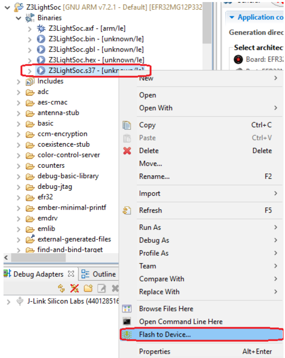
Figure 6 Select image
