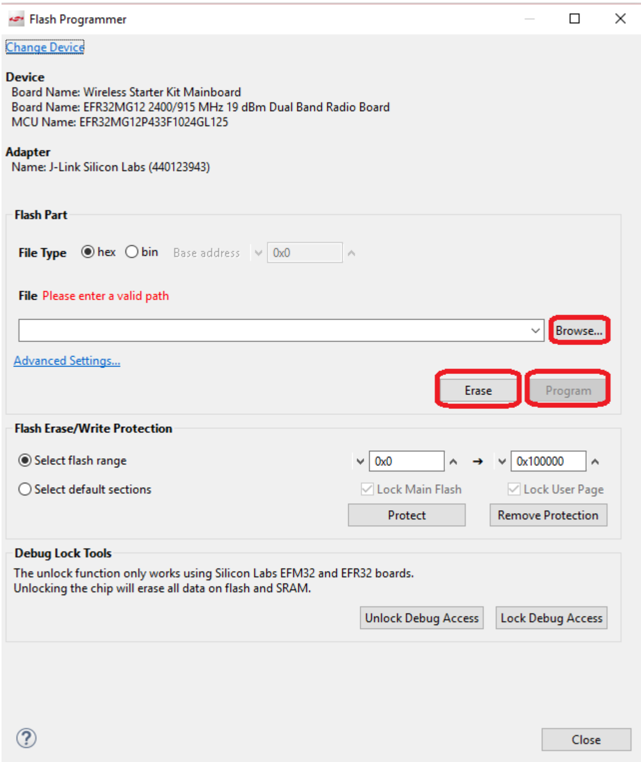
Figure 7 Flash application
