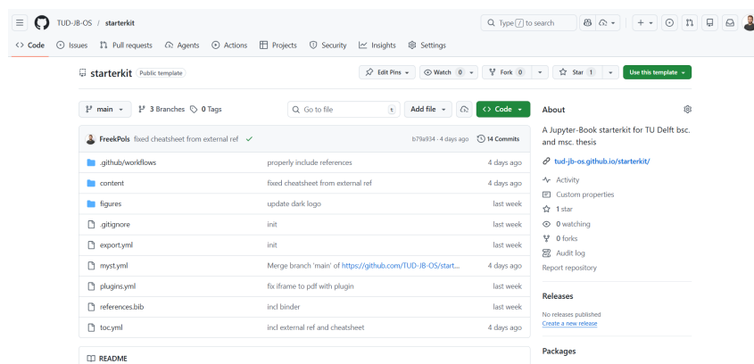
Figure 1: Folder structure.
