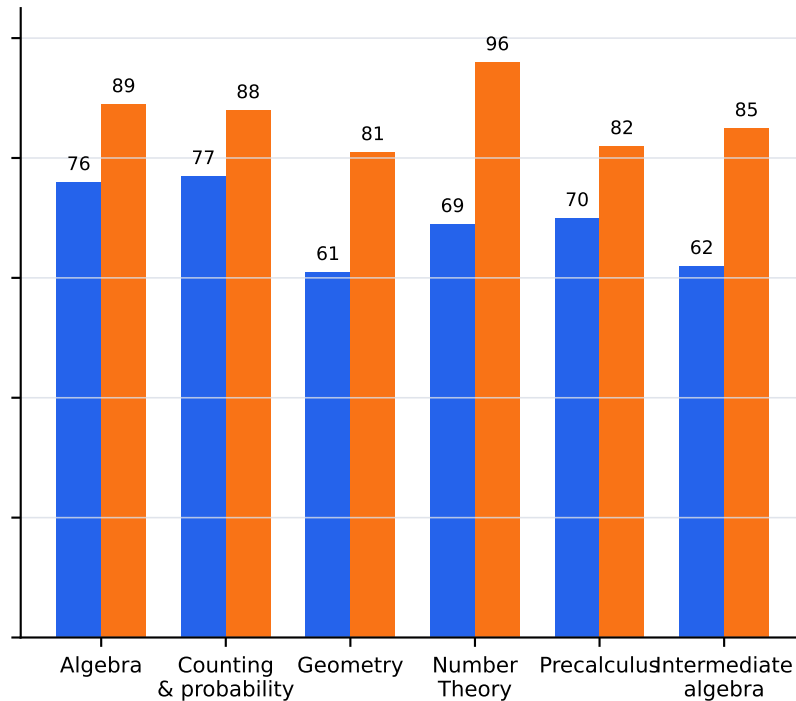
Gemini 2.5 Flash Lite
