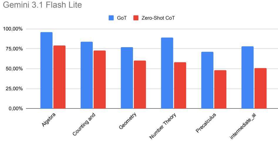
Figure 5.2: Accuracy of Gemini 3.1 Flash Lite in each category.
