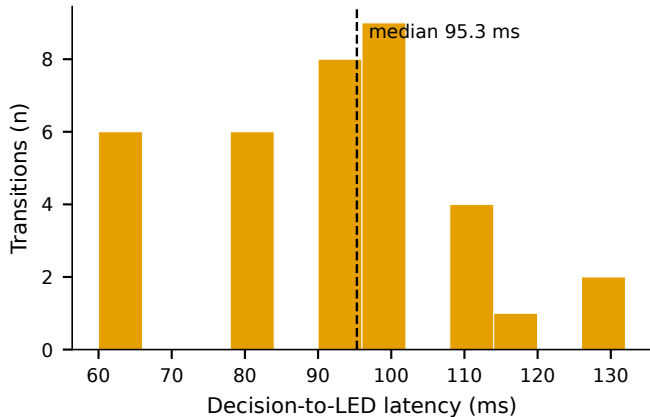
B Optical (decision → LED), n = 36 ; D = 36.4 ms
