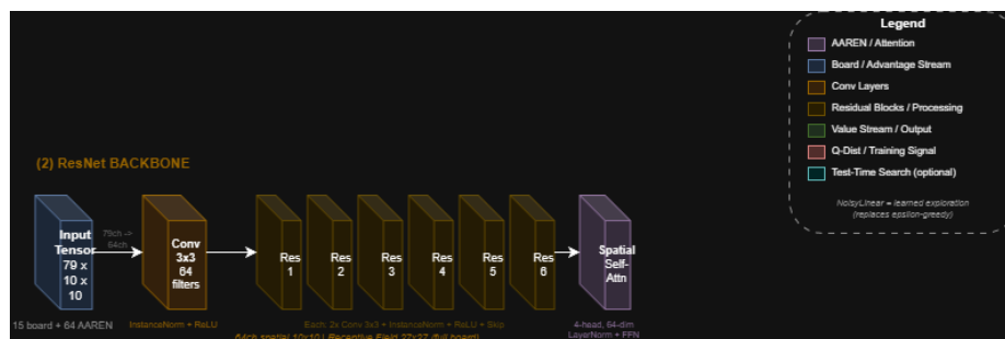
Figure 4.4: ResNet backbone.
